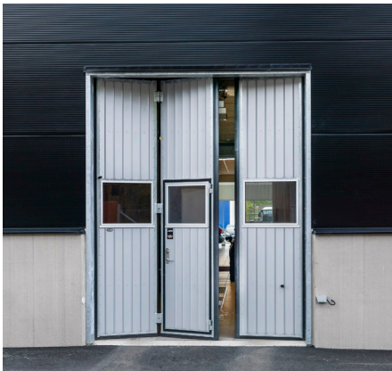
3-section folding door with recessed entrance door and a row of glass.
