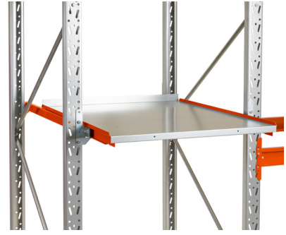
Slide-out shelf - for picking goods without pallet. Max load 300 kg.
